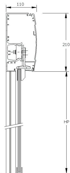
LUMINA Sans Fixe Caisson DIVA LC Standard
